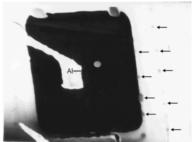
Fig.1. Microphotography of n^+ -p junction, obtained in the regime of second electrons of SEM. x1400. The point defect clusters (PDC) in space charge layer on the interface of collector-base and collector-matrix are shown by pointers. Al is the aluminium contact.
