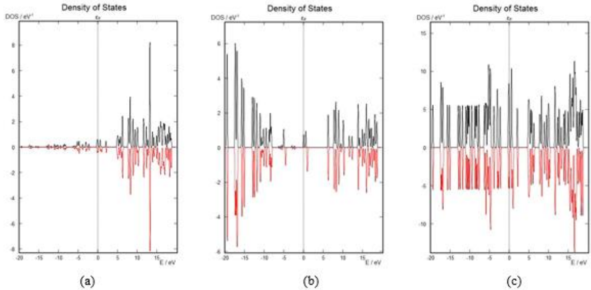
Fig. 5. The DOS for spin up and spin down d-, s-, and s p-state electrons of the dopant Ge atom and C vacancy in the 18 atoms supercell : a) d-state, b) s-state, c) s p-state
